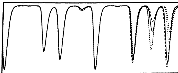
FIG. 4. Sensitivity to initial conditions in the laser with modulated parameters. Four different trajectories corresponding to nearly identical initial conditions have been plotted with different lines for a time duration of about 30 \mu s.
