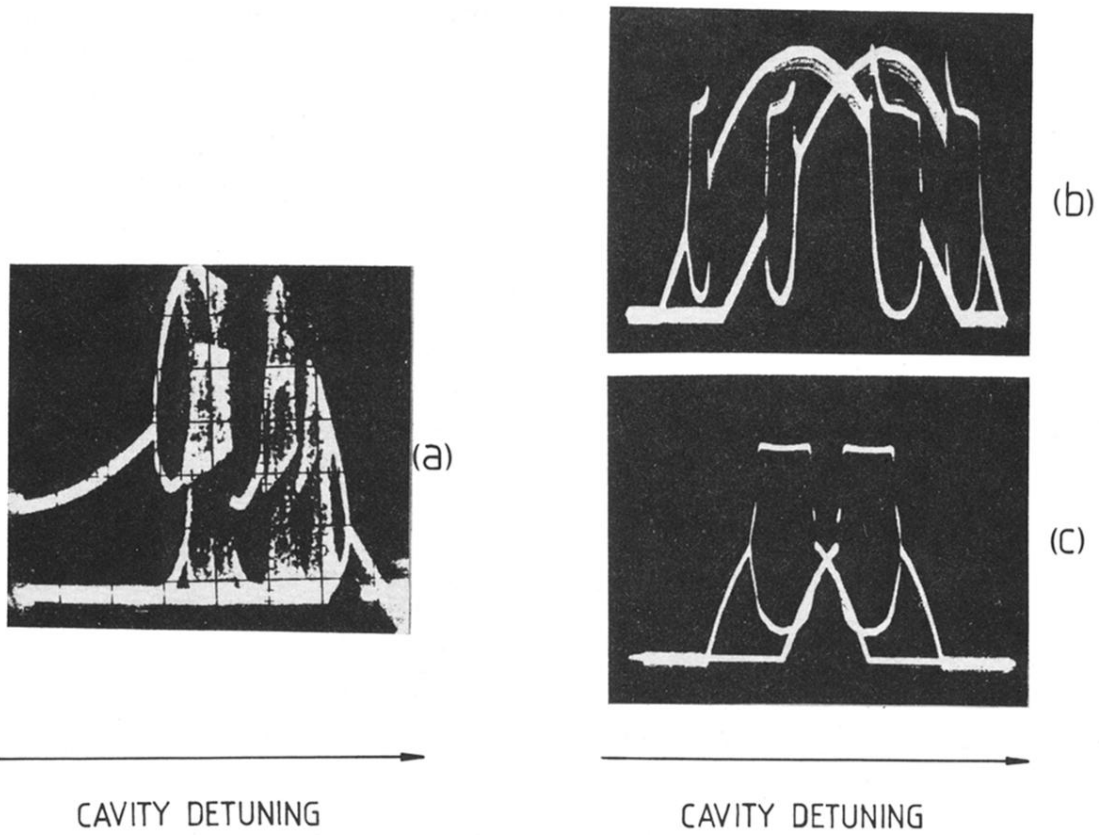
FIG. 8. Bifurcation diagrams obtained with the laser detuning as a control parameter for (a) high modulation amplitude and (b) and (c) low modulation amplitude. The most nonlinear regime has been obtained in the slope of the laser mode when the laser gain is low (c) and on top of the mode (zero detuning) when it is high (b). The detuning is swept over one mode width ( \sim 200 Mhz).
